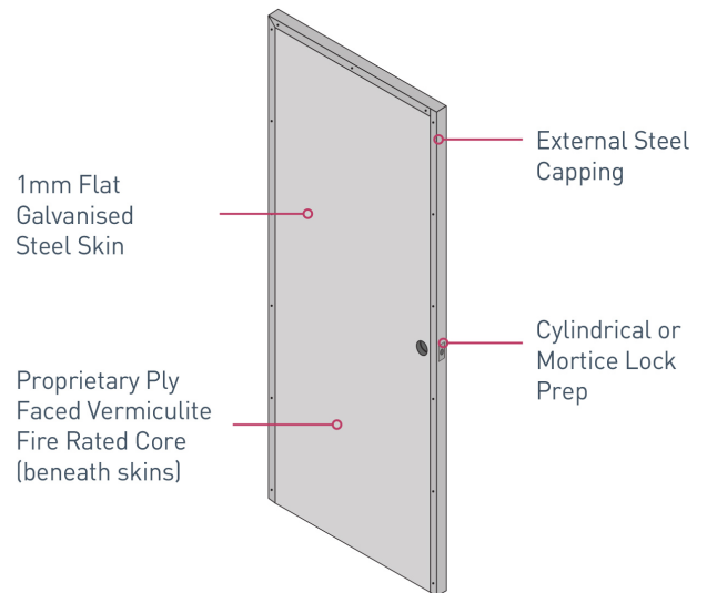
Mortice Lock Preparation Recess in steel surface allows plate of mortice lock to flush fix
