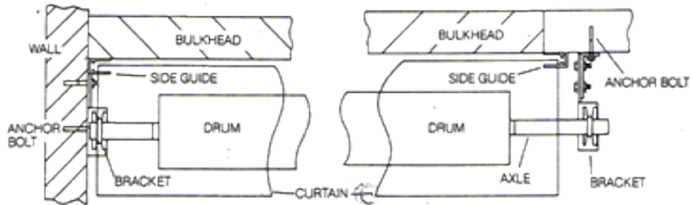
OUTSIDE JAMB FIXING
