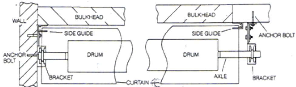
OUTSIDE JAMB FIXING
